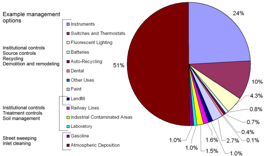
Figure 3-4. Estimated mass of Hg entering storm drains and creeks in the Bay Area. Note that the example management options will be discussed more in Section 4 of this tool box. In addition, note, that there are differing levels of confidence for each sections of the pie. The order of confidence for Hg from greatest to least is as follows: High: switches and thermostats, and fluorescent lighting, and instruments); Medium: dental, landfill, paint, laboratory, atmospheric deposition, batteries, gasoline, other uses (mainly cell phones, LCD TVs and other modern use devices), and railway lines; Low: Industrial contaminated areas and auto-recycling.
