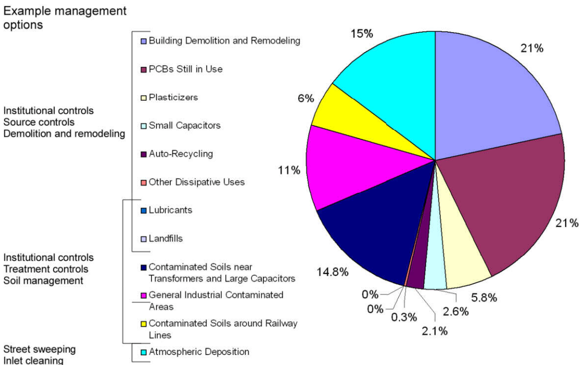
Figure 3-3. Estimated mass of PCBs entering storm drains and creeks in the Bay Area. Note, that there is differing levels of confidence for each sections of the pie. The order of confidence for PCBs from greatest to least is as follows: High: PCBs still in use, contaminated soils near transformers and large capacitors, small capacitors, other dissipative uses, plasticizers, auto-recycling, and general industrial contaminated areas; Low: building demolition and remodeling, lubricants, landfills, contaminated soils around railway lines, and atmospheric deposition.
